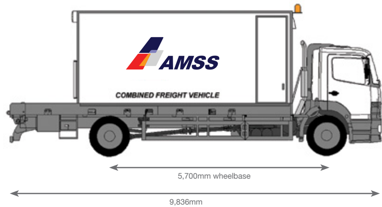
¾ box body example
